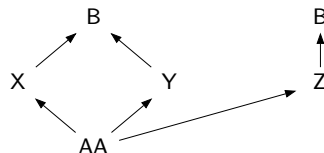
Figure 6 — Virtual and non-virtual base [fig:class.virtnonvirt]
